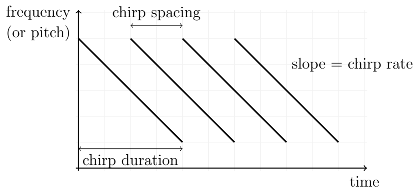
Figure 1. Conceptual time-frequency plot for the Risset glissando.
