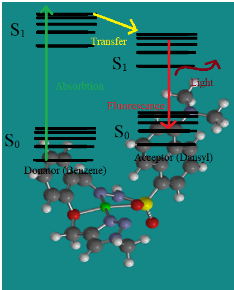
Figure 1: An example of FRET based fluorescence
